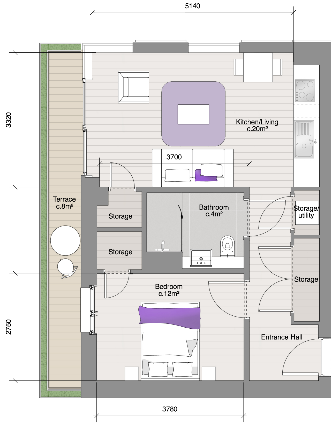
Apartment 1 | Not to scale
